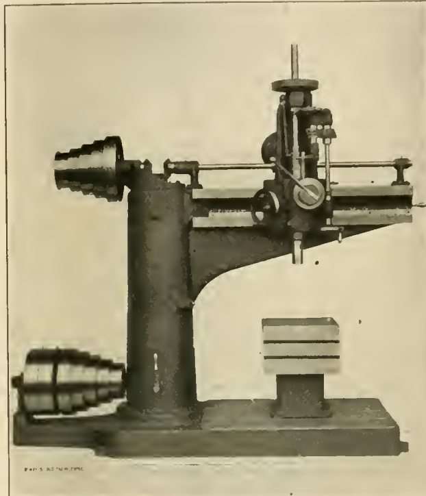
BICKFORD SEMI-RADIAL DRILL.
